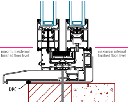
Twin track with sill
