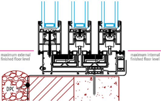
Triple track no sill
