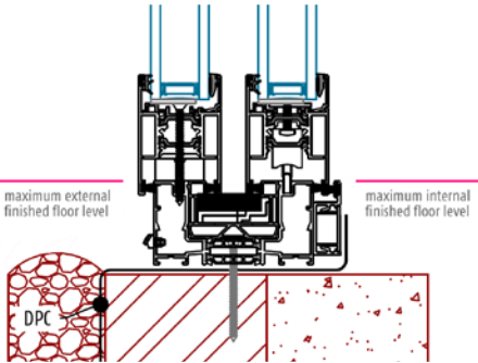
Twin track no sill
