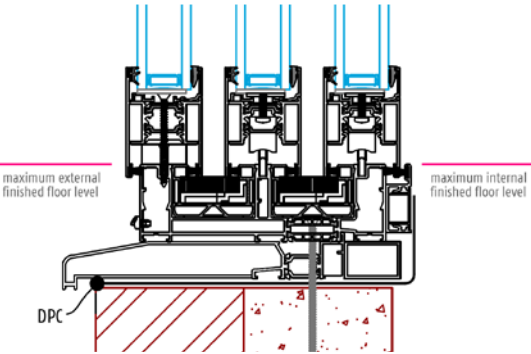
Triple track with sill
